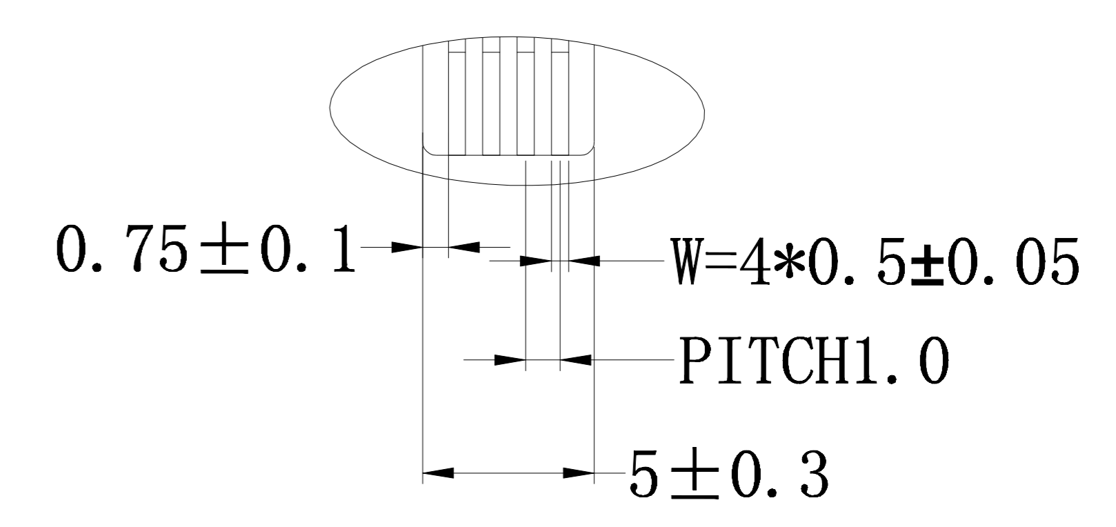
DetailA
